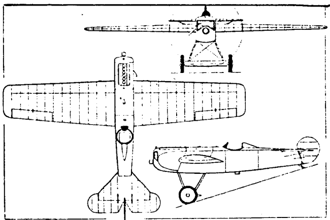
Three-view (above) and photograph of the Fokker V 21, one of the prototype monoplanes entered by Fokker in the second D-type competition in May-June 1918. The V 23 was similar but had untapered wings.
